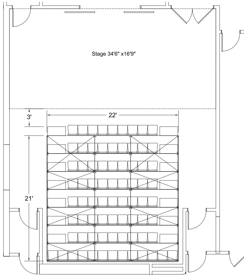
SEATING RISER LAYOUT #4 SEATS - 76
