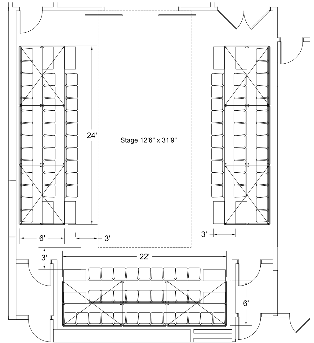
SEATING RISER LAYOUT #3 SEATS - 99
