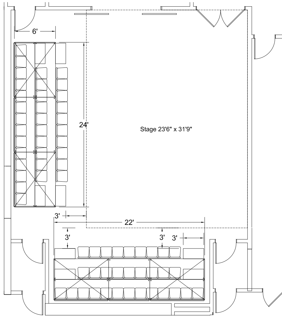
SEATING RISER LAYOUT #1 SEATS - 65
